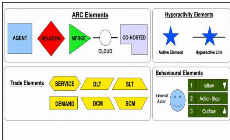
Figure 3. Key elements of the Agent Relation Charts. Image credit to [2].
