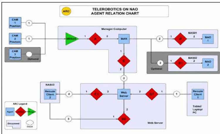
Figure 6. ARC diagram representing Structural and Relational views
