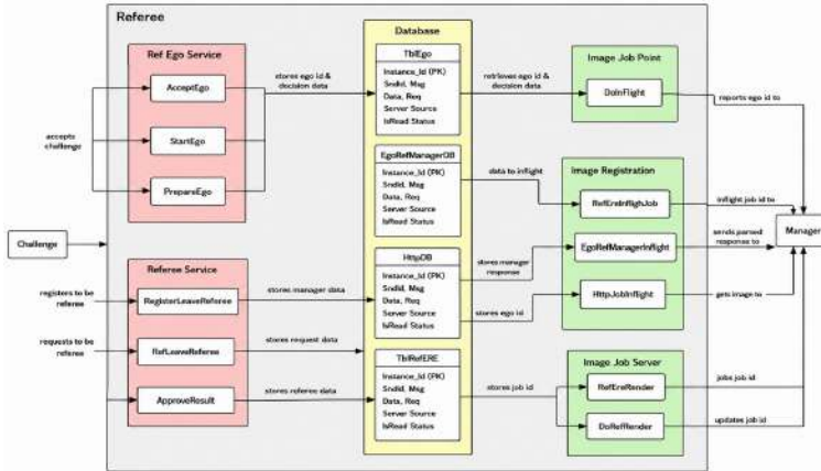
Figure 13. UML Class Diagram For Webserver Agent
