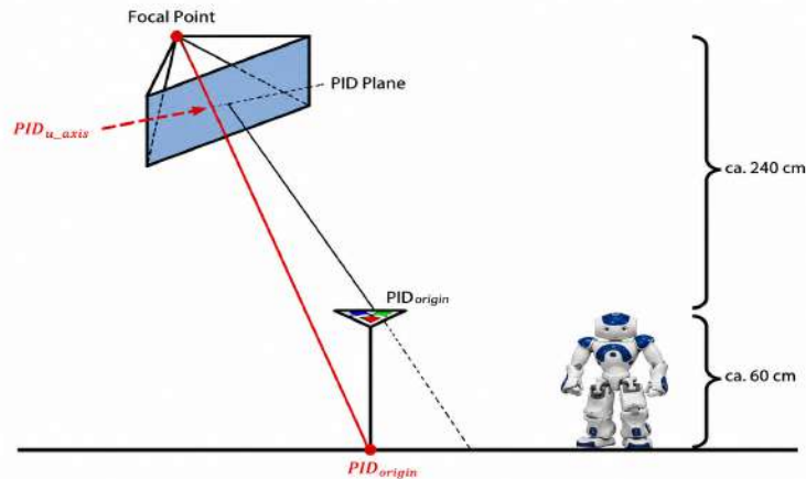
Figure 9. Schematic Workspace View Depicting The Difference Between The Detected Marker Position And The Real Robot Location
