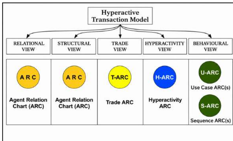
Figure 2. Five Design Views Of The ARC Meta Model. Image Credit To [2] .
