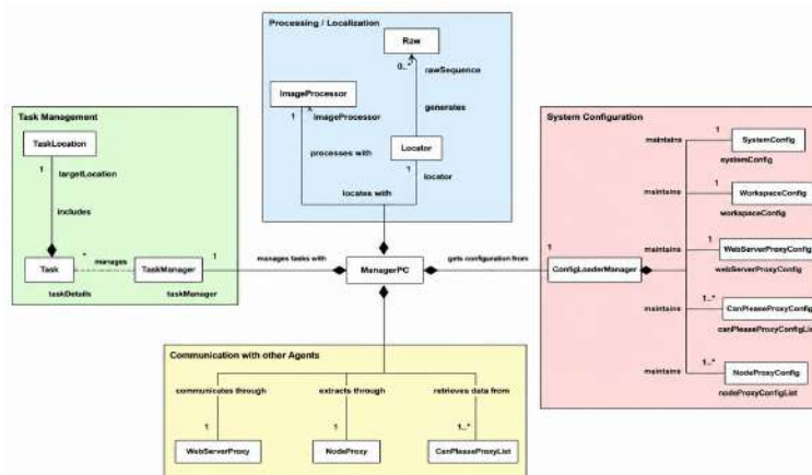
Figure 11. UML Class Diagram For Managerpc Agent
