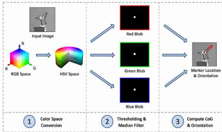
Figure 8. Marker Detection Procedure Used For Localizing Nao Within A Single Camera View
