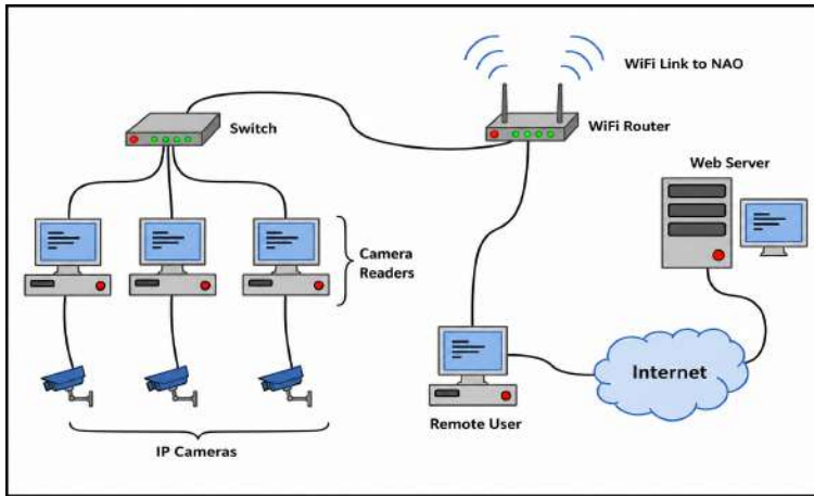
Figure 5. Overview Of The Telepresence System Depicting The Individual Agents, Hardware And Communication Lin
