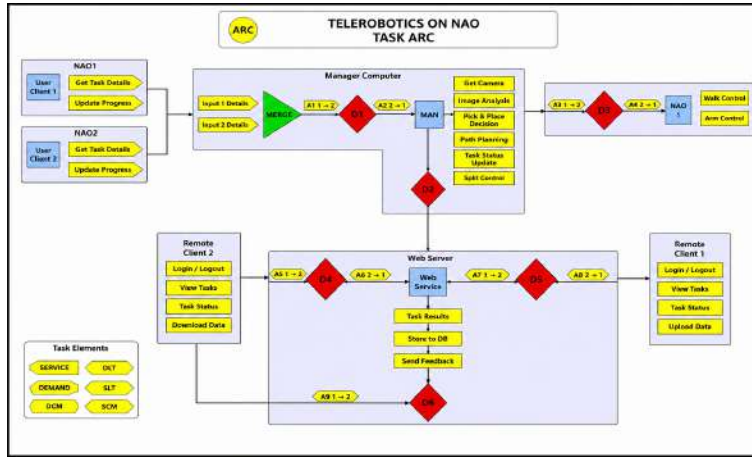
Figure 7. ARC Diagram Representing The Trade View
