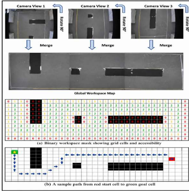
Figure 10. Composition of Global Workspace Map From Individual Views
