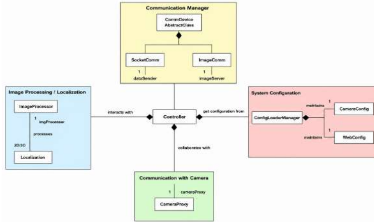
Figure 12. UML Class Diagram For Camreader Agent
