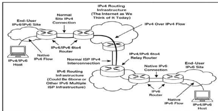
Figure 4. The 6to4 Relay
