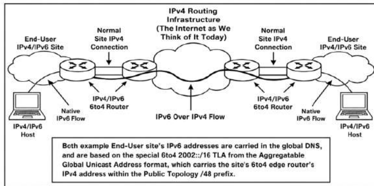
Figure 2. 6to4 Tunnel Overview
