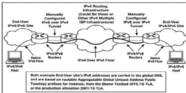
Figure 1. Configured Tunnel Overview
