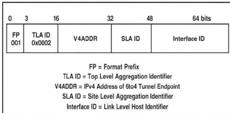
Figure 3. 6to4 Prefix Format
