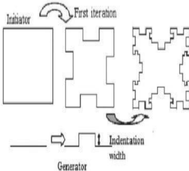
Figure 9. Several stages in the construction of a Minkowski fractal
