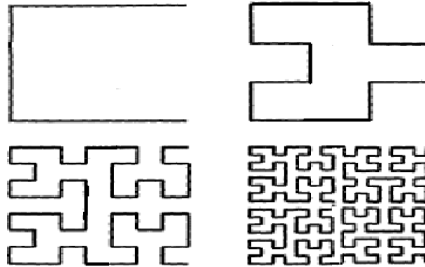
Figure 7. Several stages in the construction of a Hilbert curve
