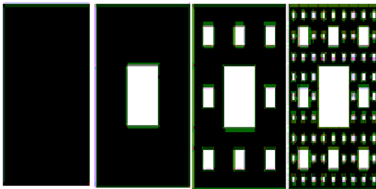
Figure 6. Sierpinski carpet fractal
