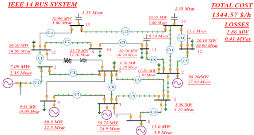
Figure 1. OPF case as minimum losses
