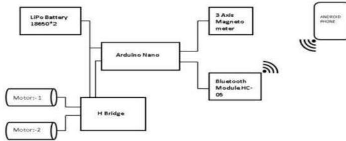
Block diagram of Bluetooth controlled robot car.
