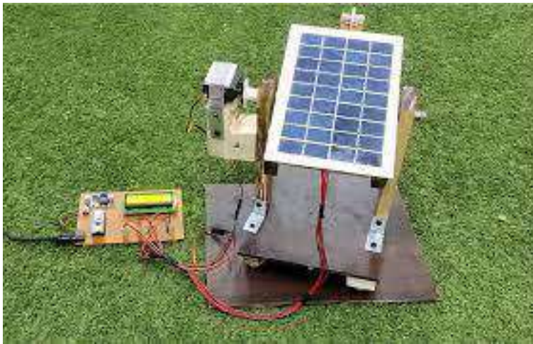
Figure 2. Prototype model
