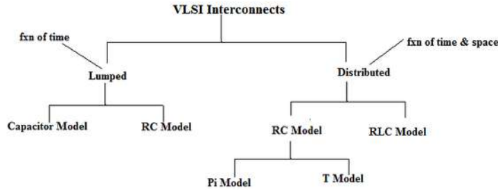
Figure 2. Various Interconnect Delay Model.
