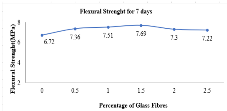
Figure 16. Flexural Strenght for 7 days
