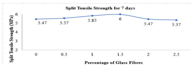
Figure 23. Split Tensile Strength for 7 days
