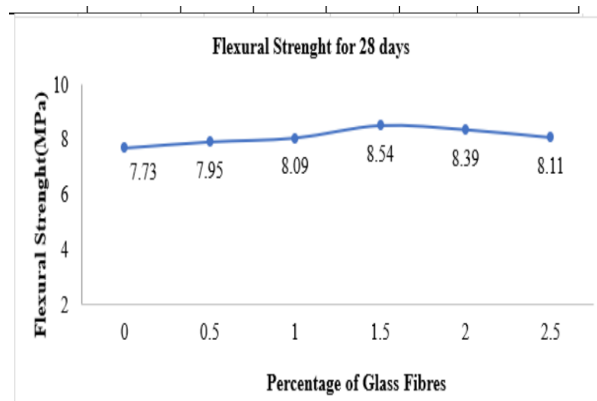
Figure 17. Flexural Strenght for 28 days
