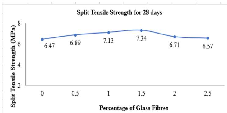
Figure 24. Split Tensile Strength for 28 days
