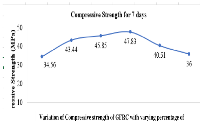
Figure 18. Compressive Strength for 7 days
