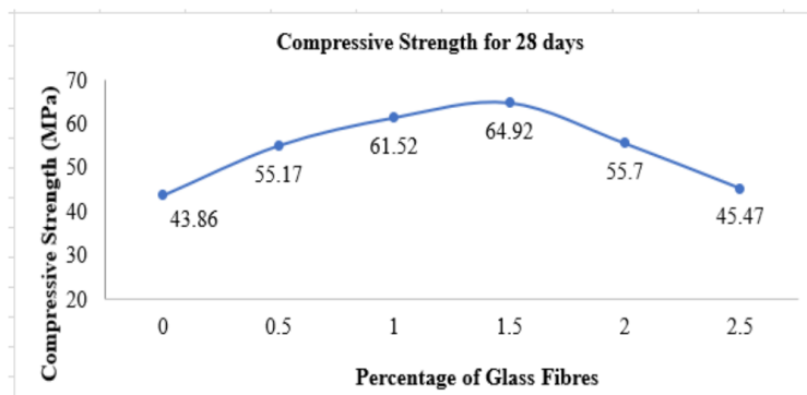
Figure 19. Compressive Strength for 28 days
