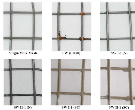
Figure 2. Specimens after 90 days of exposure (Virgin Wire Mesh, SW (Blank), SW I-1 (N), SW II-1 (N), SW I-1 (SC), SW II-1 (SC))
