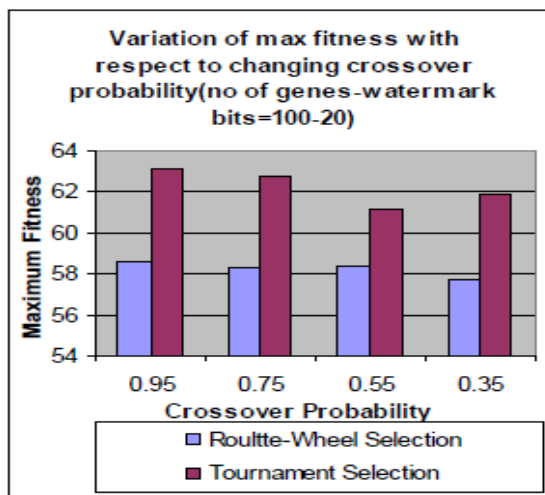
Figure 6. Variation of Maximum Fitness with Crossover Probability (no of genes-watermark bits=100-20)
