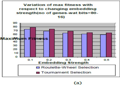
Figure 2. Variation of Maximum fitness with Embedding strength (no of genes=80, watermark bits=16)
