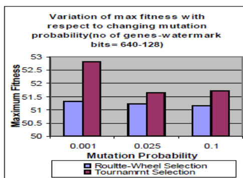
Figure 8. Variation of Maximum Fitness with Mutation Probability (no of genes-watermark bits=640-128)
