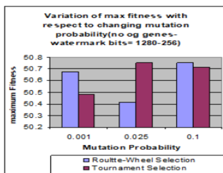
Figure 9. Variation of Maximum Fitness with Mutation Probability (no of genes-watermark bits=1280-256)
