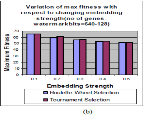
Figure 3. Variation of Maximum fitness with Embedding strength (no of genes=640, watermark bits=128)
