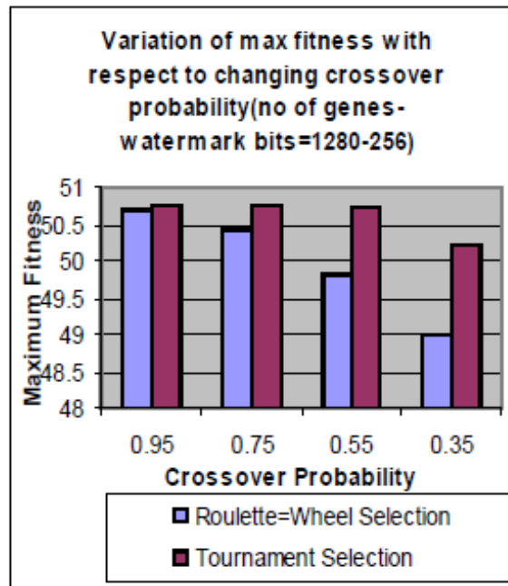
Figure 7. Variation of Maximum Fitness with Crossover Probability (no of genes-watermark bits=1280-256)
