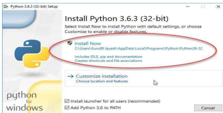
Figure 3. 6.2 Python Install
