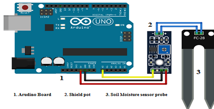
Figure 6. Connections for the Arduino based Soil Moisture sensor Interfacing Unit using YL-69 sensor probe (electrode).
