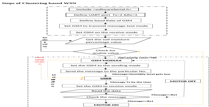
Figure 8. Flow Char of proposed Bi-directional Alerting and GSM based soil monitoring system
