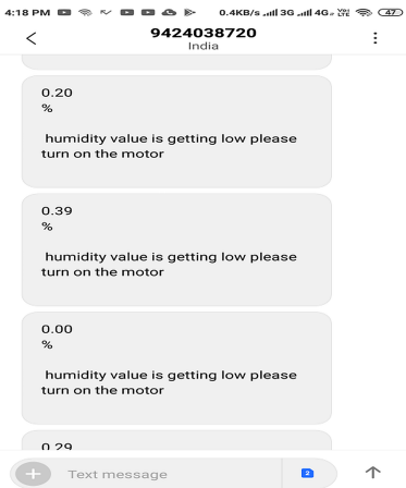
Figure 9. Result example of the percentage moisture based sent SMS sequence as mufti level GSM based text alarming system schemes.
