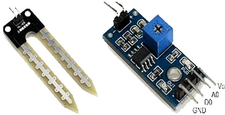
Figure 5. Basic capacitive Soil Moisture measuring sensor a) YL-69 Sensor probes or electrodes b) the Shield for interface
