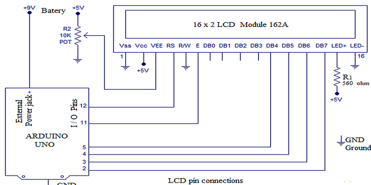
Figure 7. Circuit Layout descriptions for Arduino interfacing with LCD display [14]
