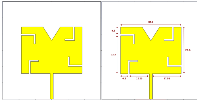
Figure 2. (a) RPA with slots (b) RPA with “L” shaped slots and dimensions
