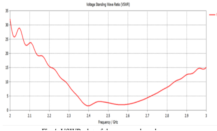
Figure 4. VSWR plot of the proposed work
