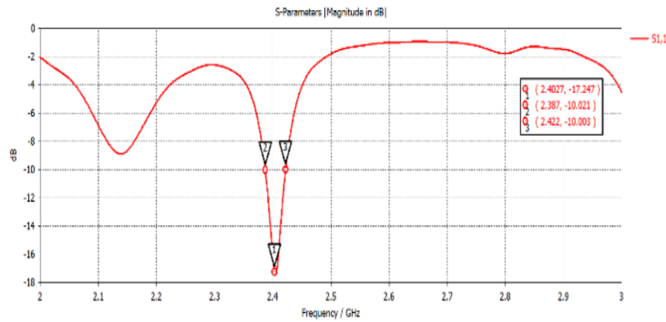
Figure 3. s11 of the proposed work
