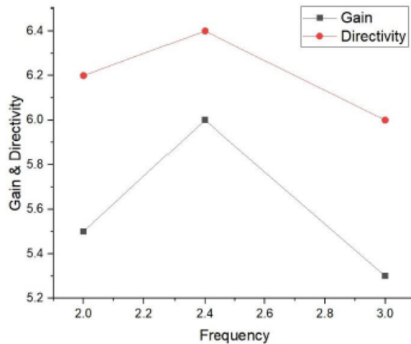
Figure 5. Gain & Directivity plot of the proposed work
