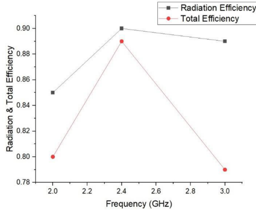
Figure 6. RE and TE plot of the proposed antenna in CST studio suite
