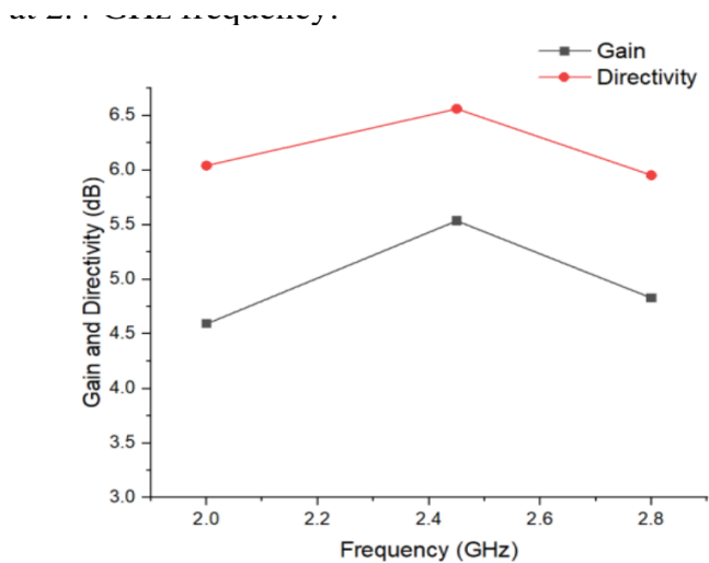
Figure 5. directivity, gain graphical plot representation projected study
