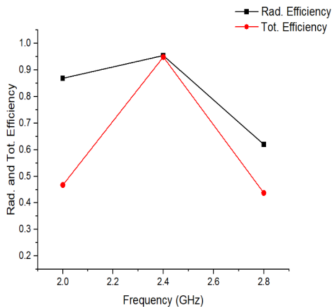
Figure 6. RE and TE graphical plot representation current study
