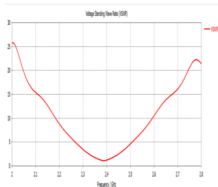
Figure 4. VSWR graphical representation of current study
