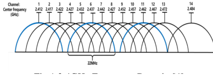
Figure 1. 2.4GHz Frequency Domain [4]
