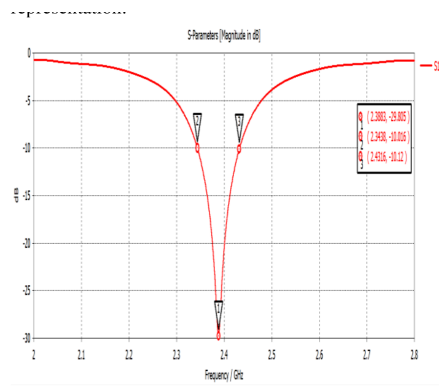
Figure 3. S11 parameters of the projected study
