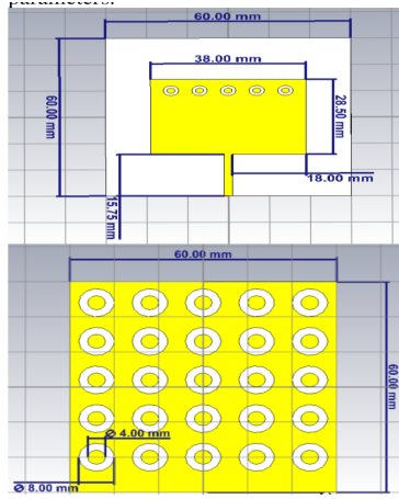
Figure 2. (a) slotted ring-shaped MPA (b) assigned antenna with DGS composition at ground
