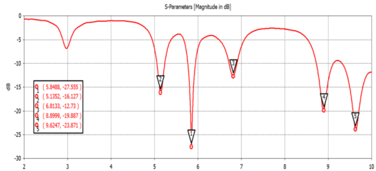
Figure 2. S11 graph of proposed work
