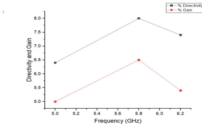
Figure 4. Antenna gain and directivity plot
