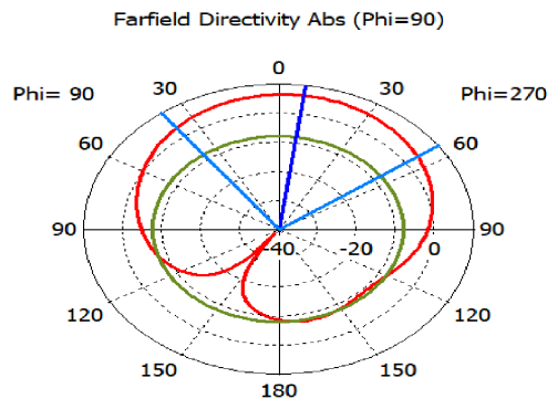
Figure 6. Far-field Rad. P for the Multiband MSP antenna
