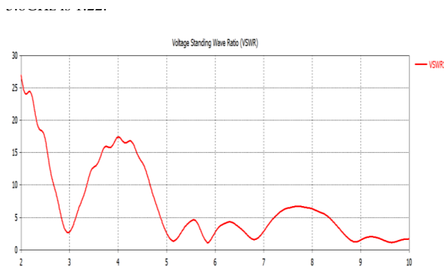
Figure 3. VSWR plot of the proposed work
