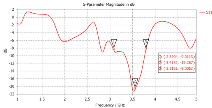
Figure 3. S11 scattered plot graph.
