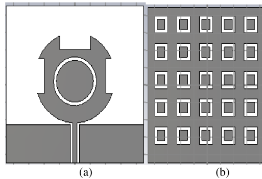
Figure 2. (a) front view of designed antenna & (b) back view with DGS.
