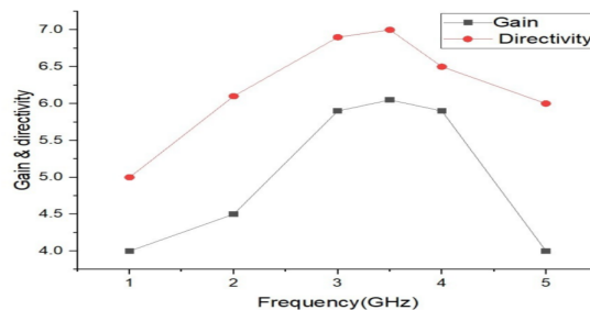
Figure 5. Intended antenna gain and directivity plot representation.
