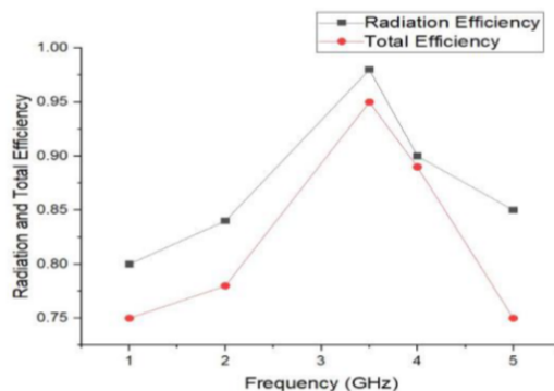
Figure 6. Radiation and Total Efficiency Plot
