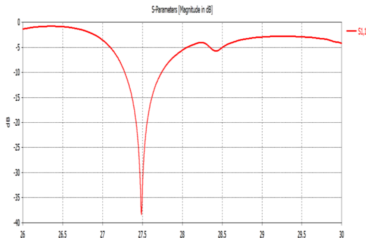
Figure 5. S_{11} of current work
