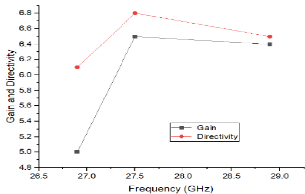
Figure 7. Gain and Directivity of current antenna
