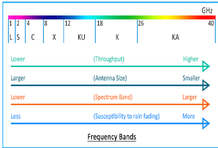
Figure 2. Satellite Frequency Band Spectrum [9]
