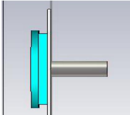
Figure 4. (b) Side view of DRA with coaxial cable
