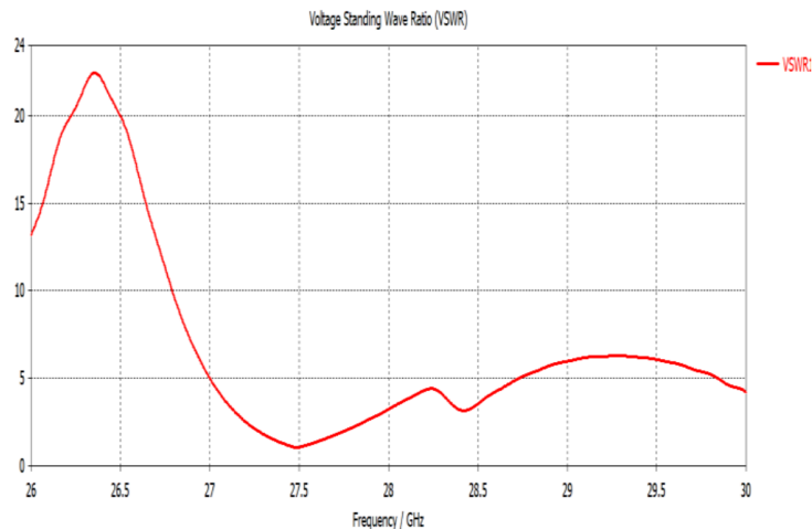
Figure 6. VSWR plot of the current work
