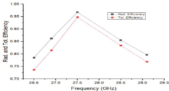
Figure 8. Radiation efficiency and Total efficiency of current antenna
