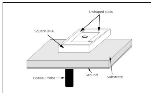
Figure 3. The projected DRA's structure
