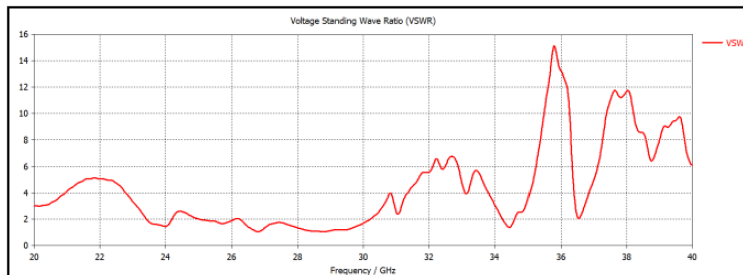
Figure 6. The projected SDR's VSWR Plot
