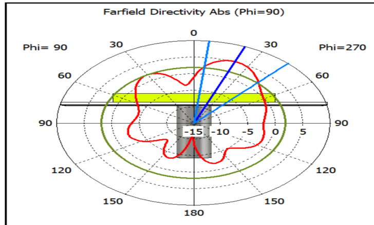
Figure 9. The projected SDRA's far-field radiation pattern
