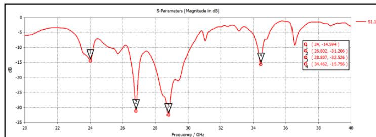
Figure 5. The projected SDR's Reflection coefficient s_{11}
