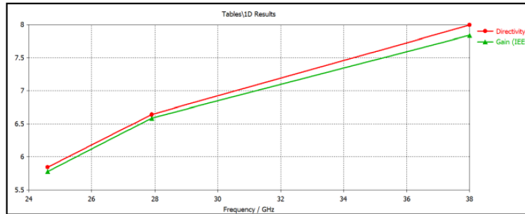
Figure 7. The projected SDRA's Directivity and Gain plot
