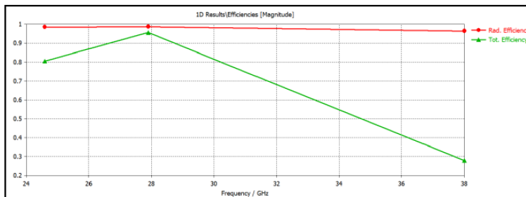
Figure 8. The projected SDRA's RE and TE plot
