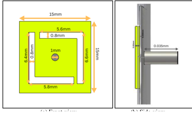
Figure 4. Dimensions of the Antenna. (a) Front-view (b) Side-view
