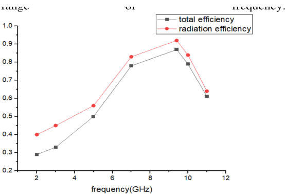
Figure 5. radiation efficiency and total efficiency plot
