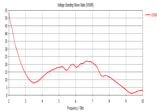
Figure 3. VSWR for the designed antenna
