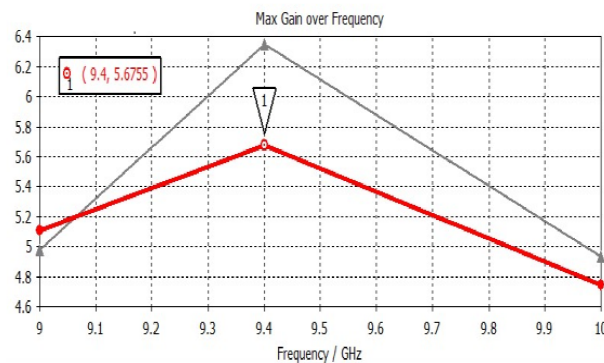
Figure 4. Gain of the designed antenna
