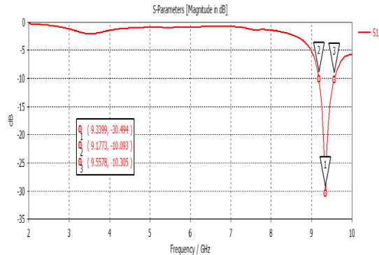
Figure 2. Reflection coefficient s_{11} of the patch antenna in CST
