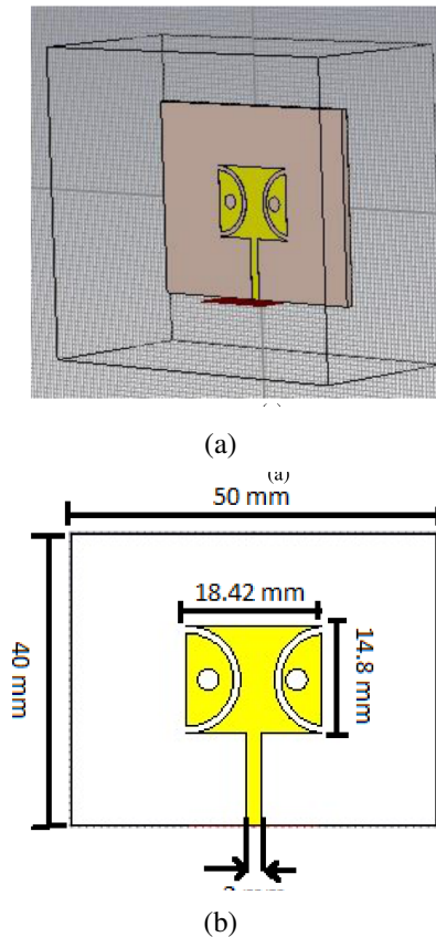
Figure 1. Rectangular microstrip patch antenna, (a) side view and (b) front view with dimensions.
