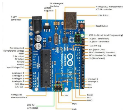
Figure 1. Arduino Uno board pin configuration
