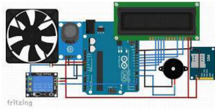
Figure 2. Proposed model of the Gas Leakage Detection System
