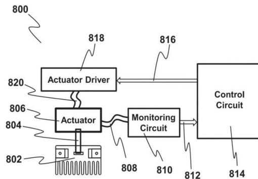
Figure 1. Block diagram of the Automated Trimmer System control architecture
