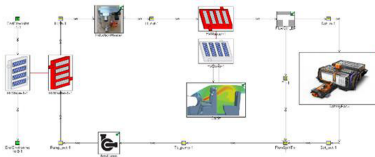
Figure 1. Simulation model of the proposed Induction Hot Pack
