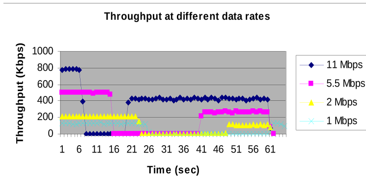
Figure 3. Effect of type2 hidden terminal on throughput
