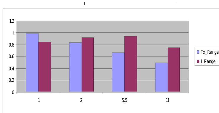
Figure 2. Tx_range and L_range comparisons of the rates in IEEE 802.11b, normalized by 1 Mbps with \alpha = 4
