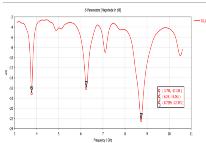
Figure 3. s_{11} Parameter of the designed antenna in CST studio suite
