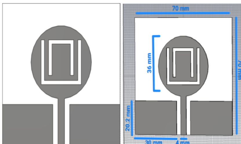
Figure 2. (a) Circular MPA & (b) proposed antenna with CPW feeding and dimensions
