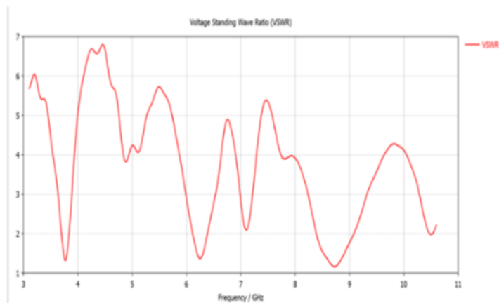
Figure 4. VSWR plot of the designed antenna
