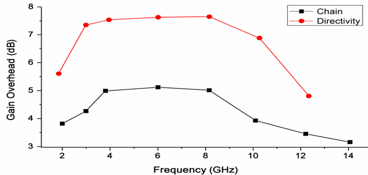
Figure 5. Proposed antenna gain and directivity plot
