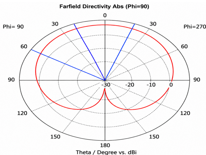
Figure 7. Presented antenna's far-field emission plot
