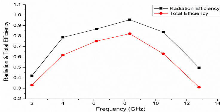
Figure 6. Proposed antenna radiation and total efficiency plot
