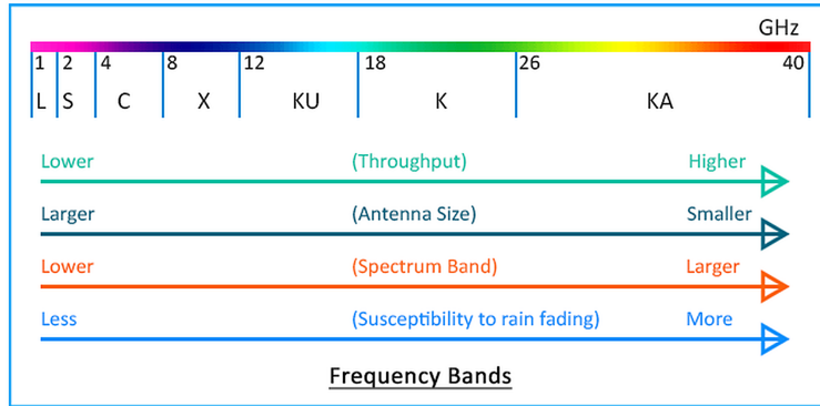
Figure 2. Satellite Frequency Band Spectrum [9]
