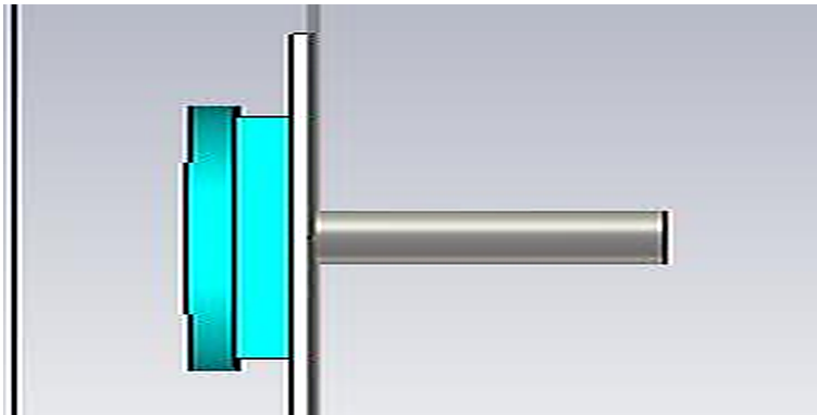
Figure 4. (b) Side view of DRA with coaxial cable
