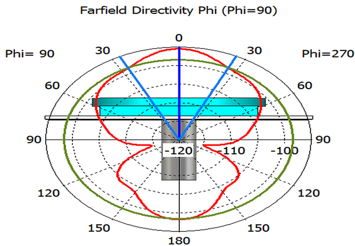
Figure 9. Radiation pattern of current work
