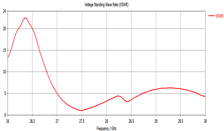
Figure 6. VSWR plot of the current work
