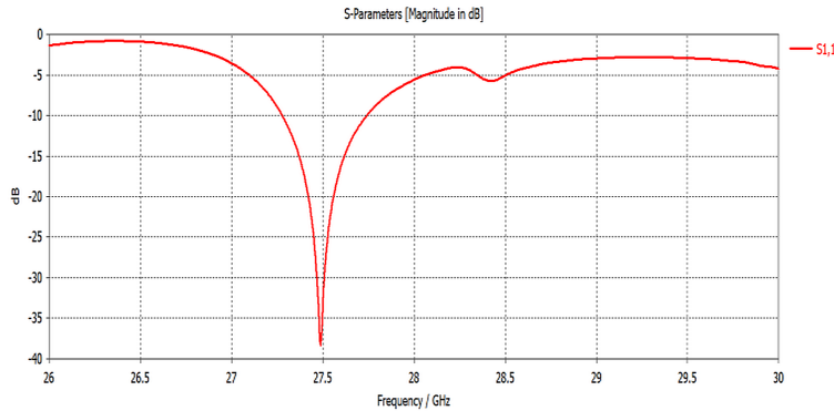
Figure 5. S_{11} of current work
