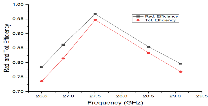
Figure 8. Radiation efficiency and Total efficiency of current antenna
