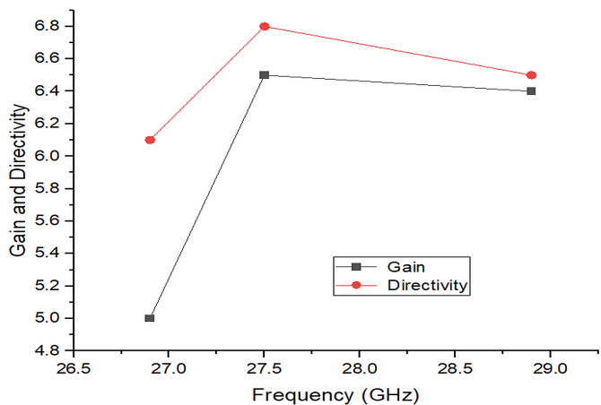
Figure 7. Gain and Directivity of current antenna
