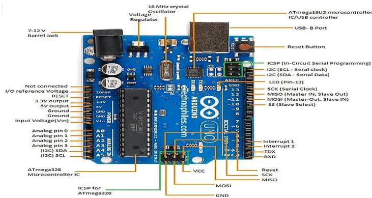
Figure 1. Arduino Uno Board
