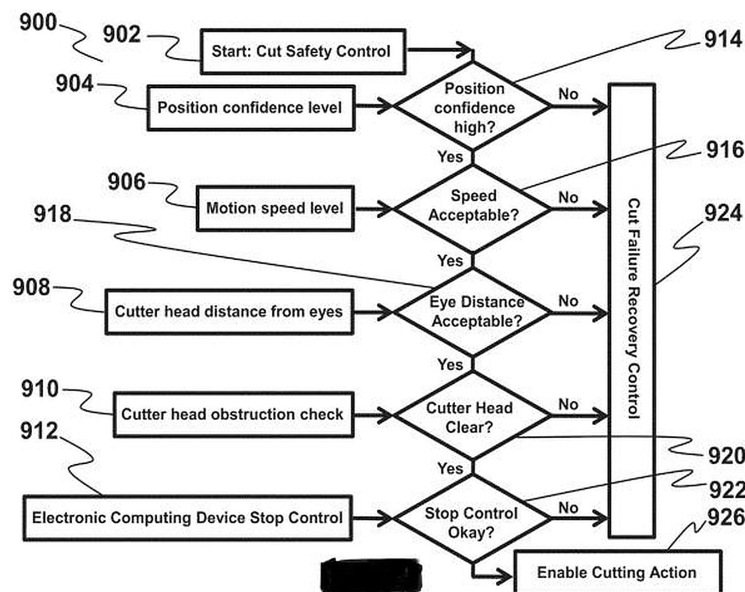
Figure 2. Cut safety control and cut failure recovery control flow of the Automated Trimmer System
