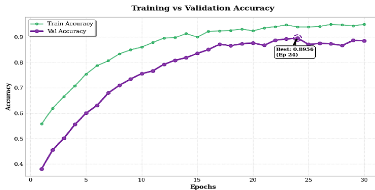
Figure 5. Training and Validation Accuracy Curves of the EfficientNetB0 Model
