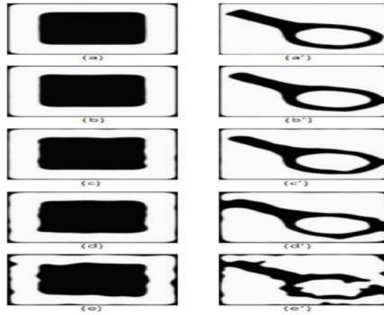
Figure 6. Extracted uniform noise affected images using MLSONN (a)(b)(c)(d)(e) Synthetic image at \epsilon=64\% , 100%, 144%, 196% and 256%; (a')(b')(c')(d')(e') Extracted Gaussian noise affected images using MLSONN (a)(b)(c)(d)(e) Synthetic image at \sigma=8 10, 12, 14 and 16; (a')(b')(c')(d')(e') Real life Spanner image at \sigma=8 , 10, 12, 14 and 16.
