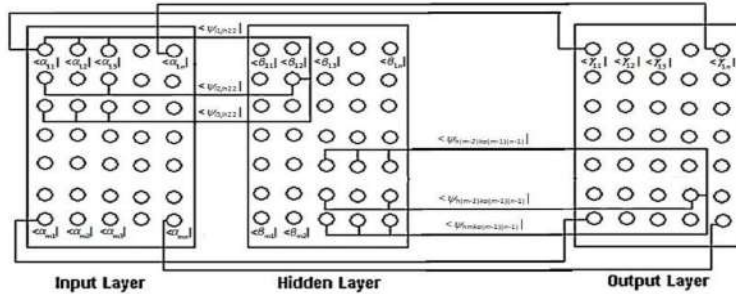
Figure 1. Schematic of a QMLSONN. Only few interconnections are shown for the sake of clarity.
