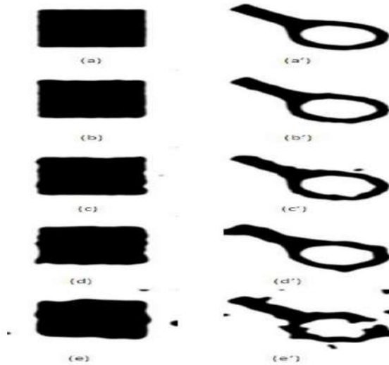
Figure 8. Extracted uniform noise affected images using QMLSONN (a)(b)(c)(d)(e) Synthetic image at \epsilon=64\%, 100\%, 144\%, 196\% and 256\% ; (a')(b')(c')(d')(e') Real life Spanner image at \epsilon=64\%, 100\%, 144\%, 196\% and 256\%
