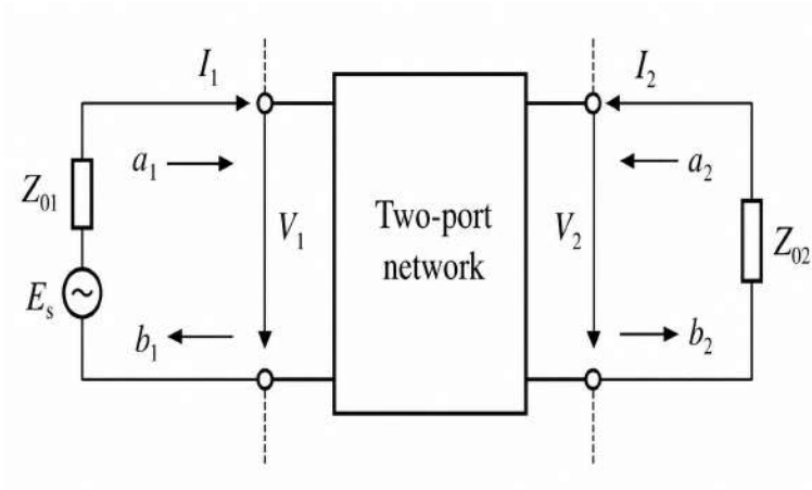
Figure 2. Two-Port Network Showing Network Variables
