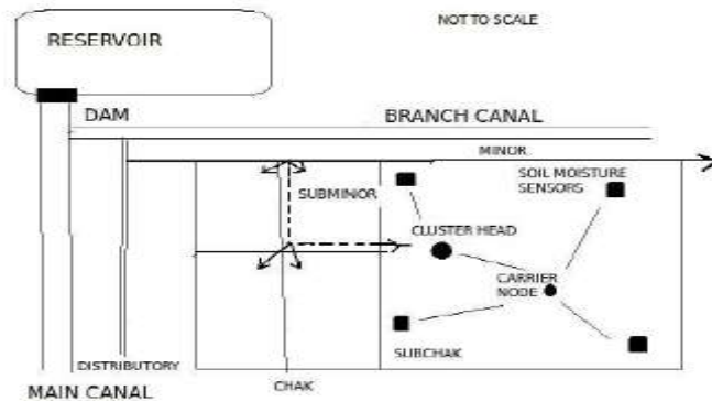
Figure 1. A Standard Irrigation Project
