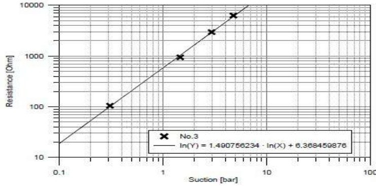
Figure 4. suction vs. electrical resistance
