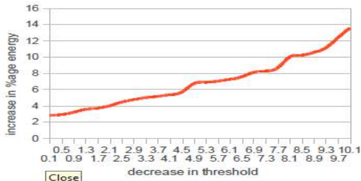
Figure 9. Increase in the energy consumption vs %age decrease in threshold
