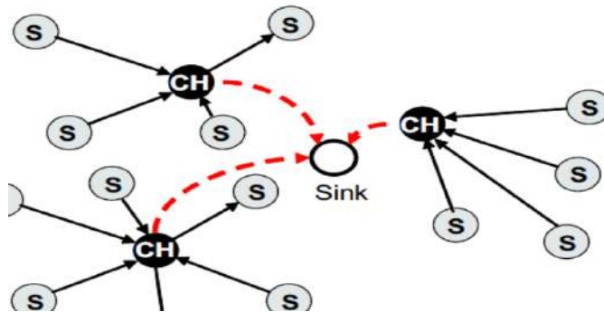
Figure 6. The cluster head routing using Leech
