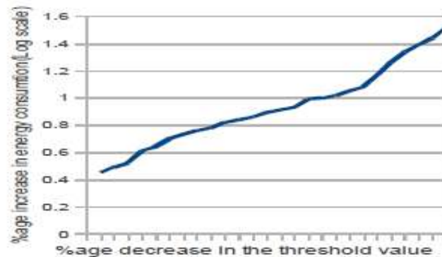
Figure 10. Decrease in the energy consumption vs %age decrease in threshold
