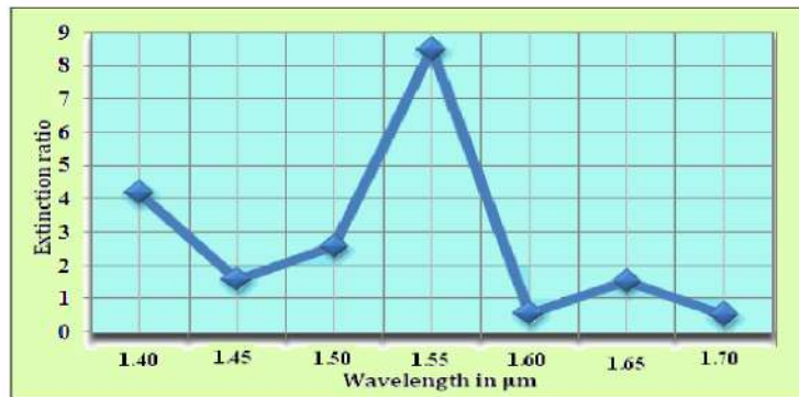
Figure 11. 5(b): Extinction ratio for different wavelength.
