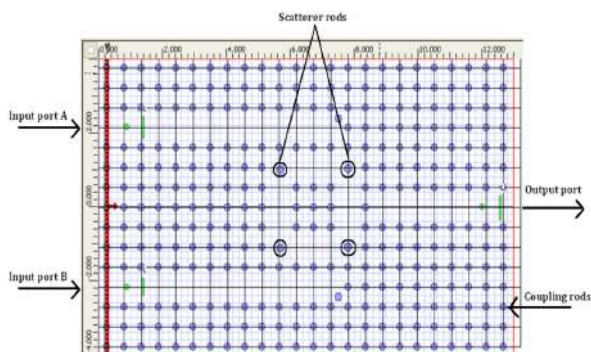
Figure 2. Design of two dimension photonic crystal based All-optical AND logic gate in X-Z plane using optiFDTD.
