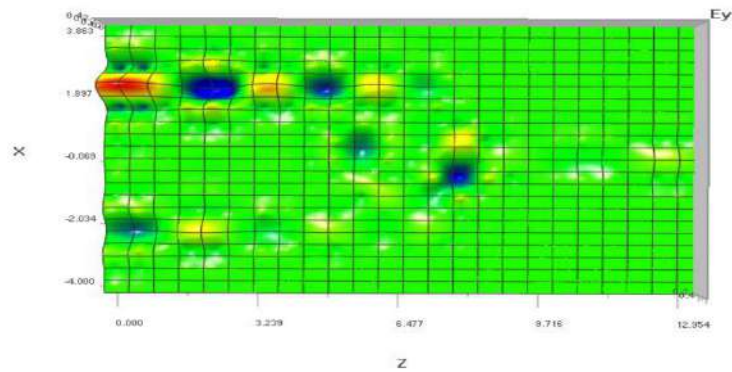
Figure 6. 4.2(a): Electric Field distributions for All-optical AND logic gate When A=1 , B=0 .
