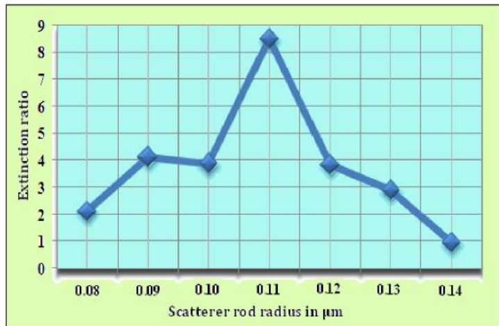
Figure 10. 5 (a): Extinction ratio for different scatterer rods radius.
