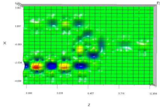
Figure 8. 4.3(a): Electric Field distributions for All-optical AND logic gate. When A=0, B=1.
