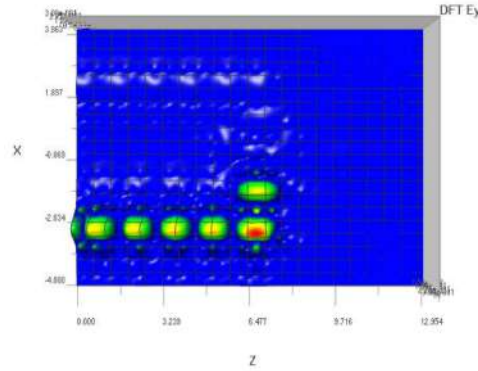
Figure 9. 4.3(b): DFT of All-optical AND logic gate: When A=0, B=1.
