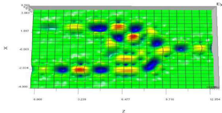
Figure 4. (a) Electric Field distributions for All-optical AND logic gate. When A=1, B=1.
