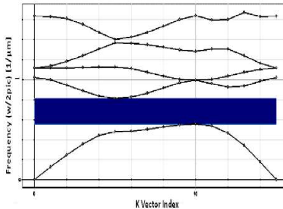
Figure 1. Band gap for AND logic gate without defect for TE mode.
