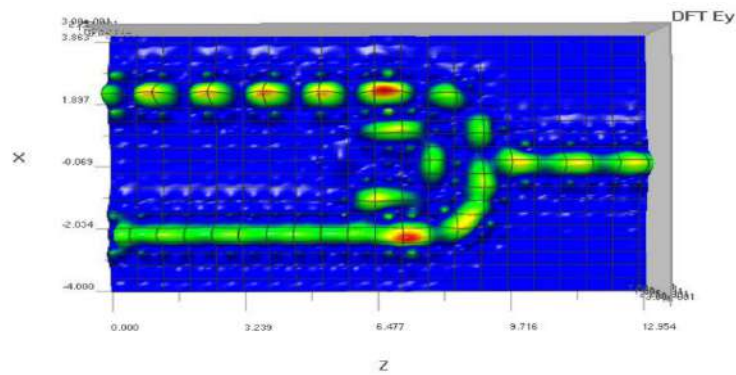
Figure 5. (b): DFT of All-optical AND logic gate: When A=1 , B=1 .
