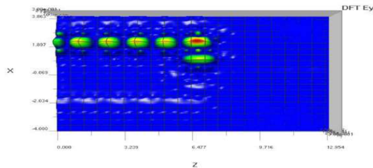
Figure 7. 4.2(b): DFT of All-optical AND logic gate: When A=1 , B=0 .
