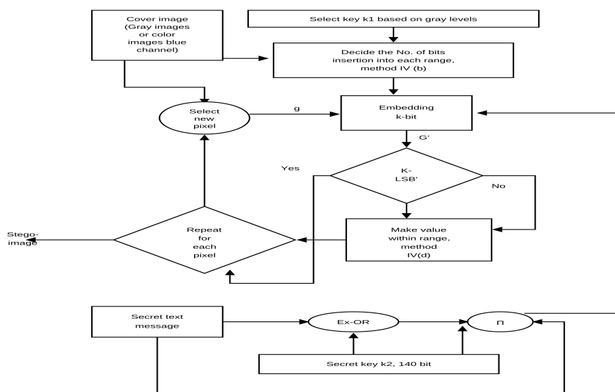
Figure 4. Message embedding with signature
