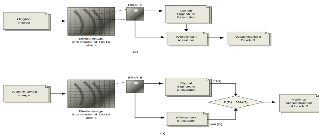
Figure 1. Watermarking insertion and extraction system. [2]
