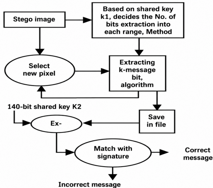
Figure 5. Messaga extraction and integrity check
