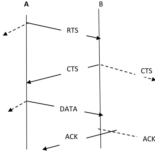
Fig. 3 Timing Diagram of Control Signals
