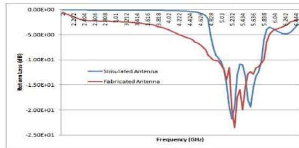
Figure 12. Comparison of return loss of simulated and fabricated antenna
