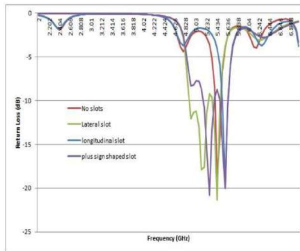
Figure 2. Effect of adding slots on the antenna
