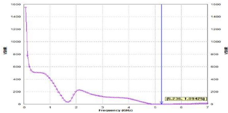
Figure 5. VSWR of proposed antenna with finite ground plane
