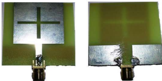
Figure 10. Front and back view of the fabricated antenna
