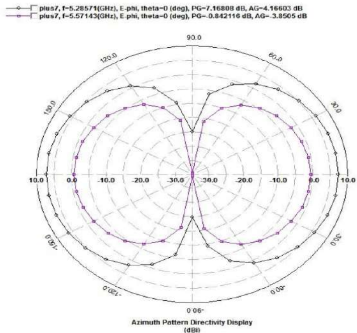
Figure 9. Azimuth pattern of proposed antenna with finite ground plane
