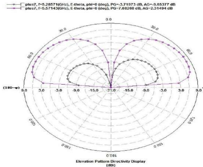
Figure 7. Directivity of proposed antenna with finite ground plane
