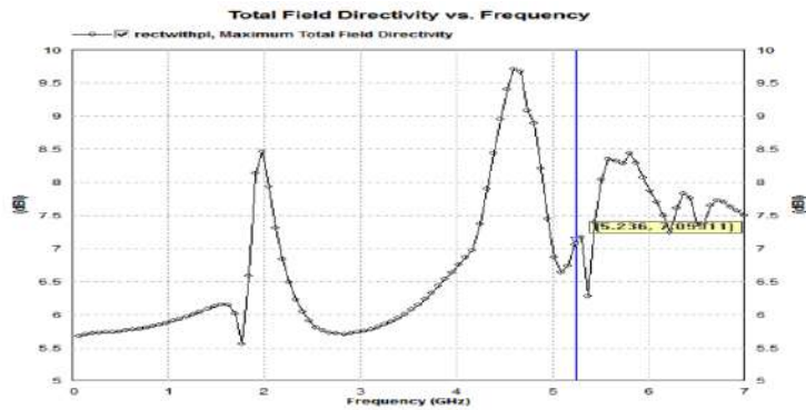
Figure 6. Gain of proposed antenna with finite ground plane
