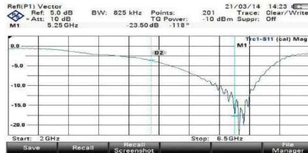
Figure 11. Return loss of the fabricated antenna
