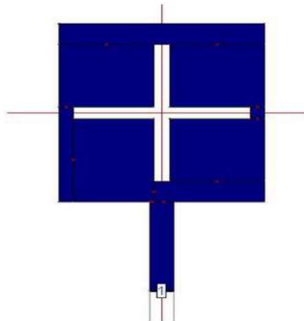
Figure 1. Proposed antenna with infinite ground plane
