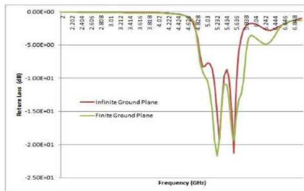
Figure 4. Return loss of proposed antenna with finite ground plane
