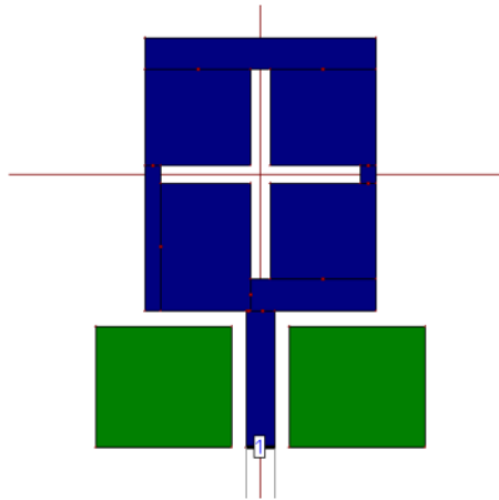
Figure 3. Geometry of proposed antenna with DGS
