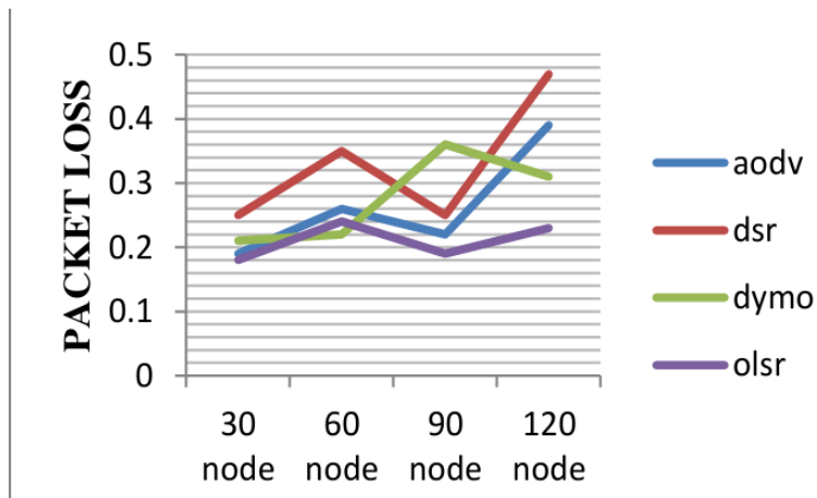
Figure 2. Packet loss for CBR Traffic with varying Node Density
