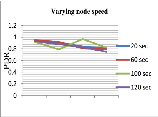
Figure 5. Effect of changing pause times on CBR in terms of PDR
