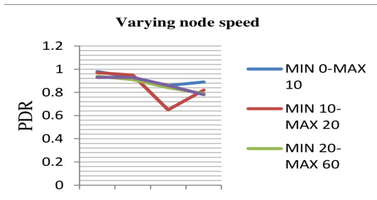
Figure 3. PDR of CBR traffic with varying speed of nodes
