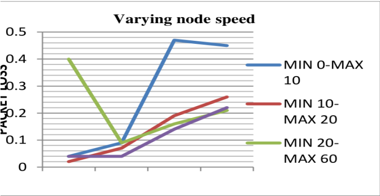
Figure 4. PL of CBR traffic with varying speed of nodes
