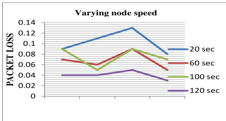
Figure 6. Effect of changing pause times on CBR in terms of PL
