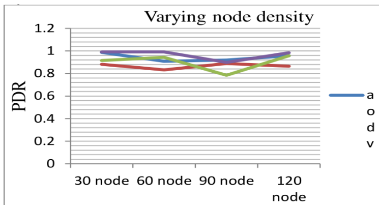
Figure 1. Packet Delivery Ratio for CBR Traffic with varying Node Density
