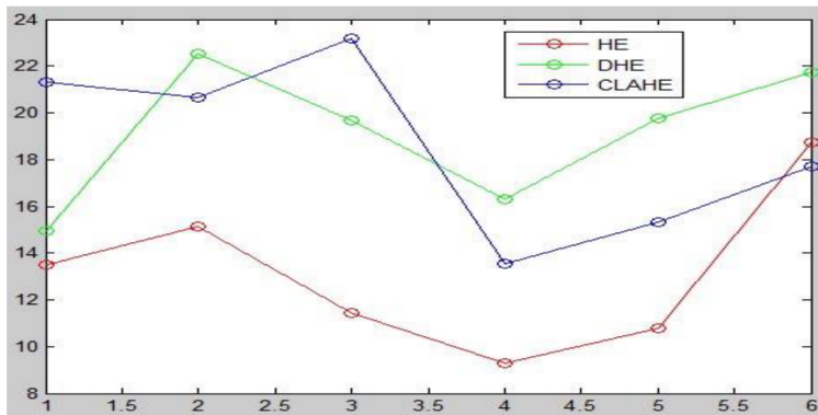
Figure 7. Illustration of the PSNR graph for various techniques for contrast enhancement.
