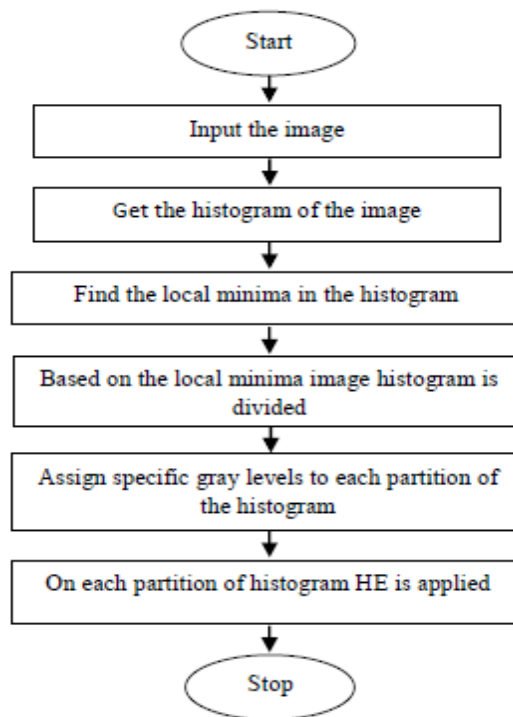
Figure 2. Flow diagram for DHE Method.
