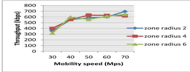
Figure 1. Impact of mobility speed on Throughput for different Zone Radius
