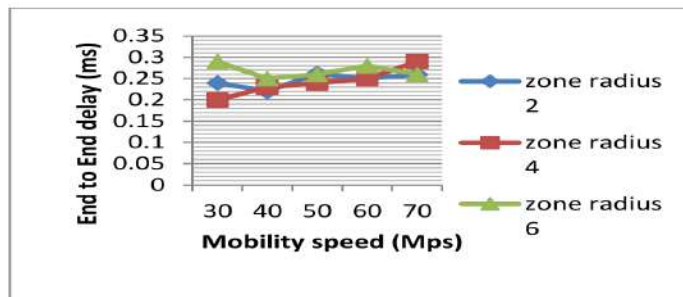
Figure 3. Impact of mobility speed on the Avg. delay for different Zone Radius
