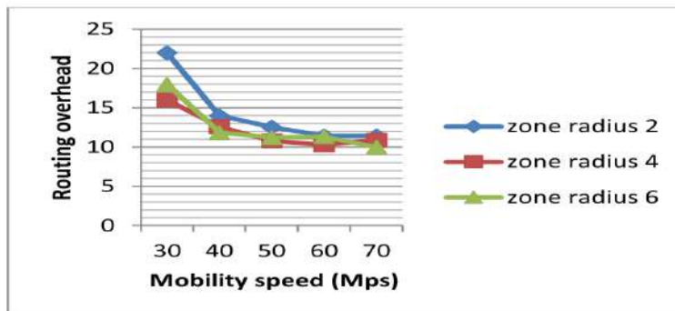
Figure 4. Impact of mobility speed on the routing overhead for different Zone Radius
