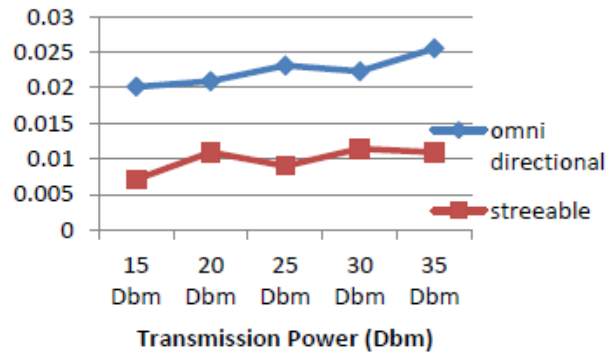
Figure 4. Average Jitter with Varying Transmission Power
