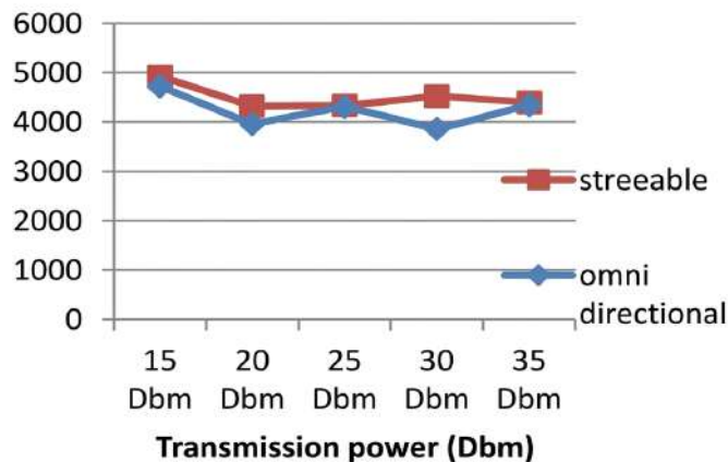
Figure 2. Throughputs with Varying Transmission Power
