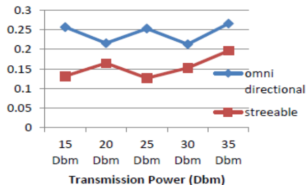
Figure 3. End To End Delays with Varying Transmission Power
