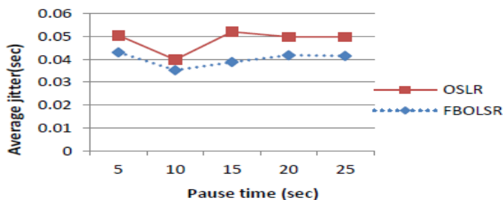
Figure 10. Average Jitter of OLSR and FBOLSR
