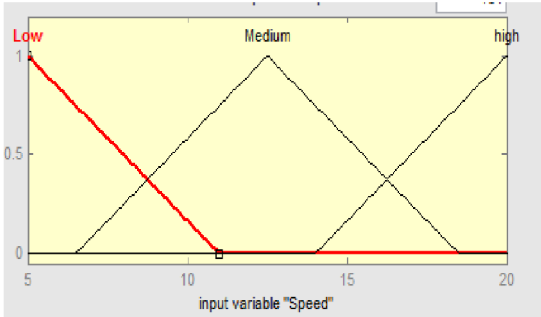
Figure 3. Membership function plot of Speed
