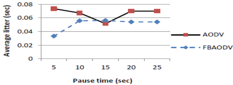
Figure 7. Average Jitter of AODV and FBAODV.
