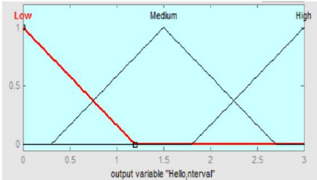
Figure 5. Membership function plot of Hello interval
