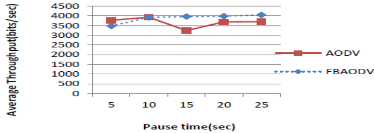
Figure 6. Average Throughput of AODV and FBAODV
