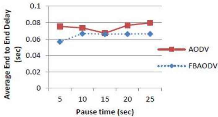
Figure 8. Average End to end delay of AODV and FBAODV
