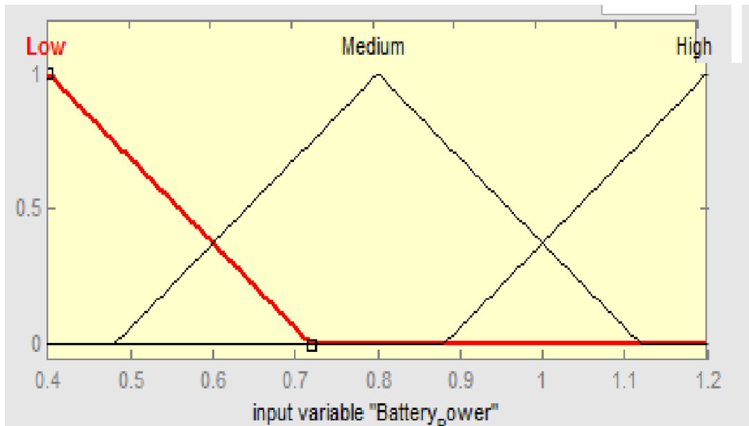
Figure 4. Membership function plot of Battery Power
