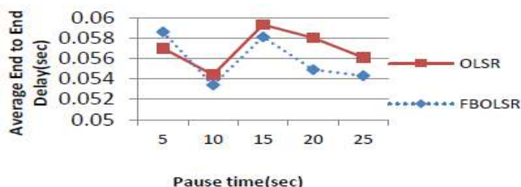
Figure 11. Average End to end Delay of OLSR and FBOLSR
