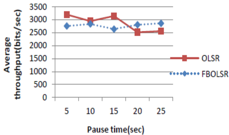
Figure 9. Average Throughput of OLSR and FBOLSR
