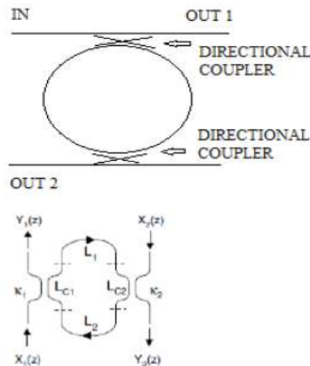
Figure 3. Simplest Optical Waveguide Filter using a Ring Resonator with Two Couplers.
