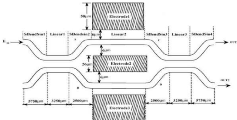
Figure 2. Schematic view of Mach–Zehnder interferometer.
