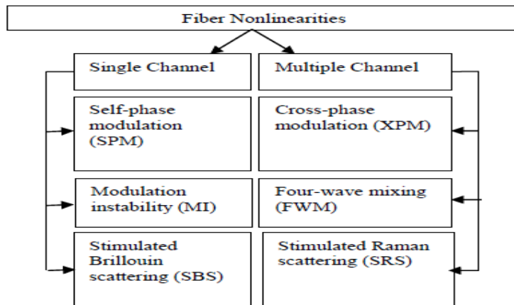
Figure 4. Fiber Nonlinearities
