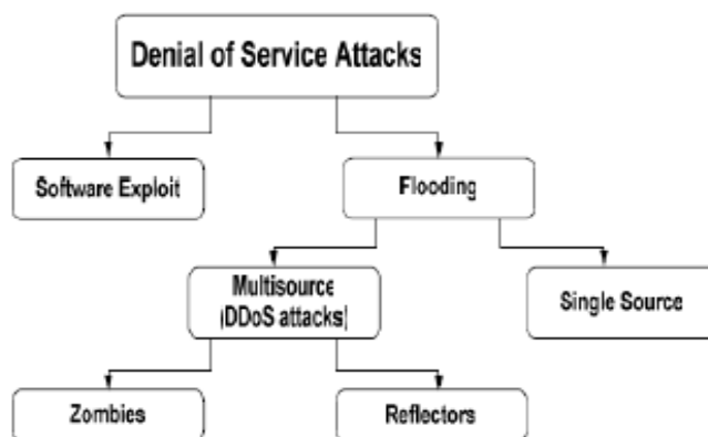
Figure 3. A basic DOS attack taxonomy
