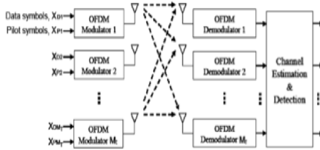
Figure 2. Block Diagram of MIMO OFDM System
