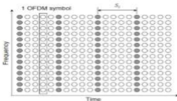
Figure 3. Blok type pilot arrangement
