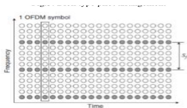
Figure 4. Comb type pilot arrangement
