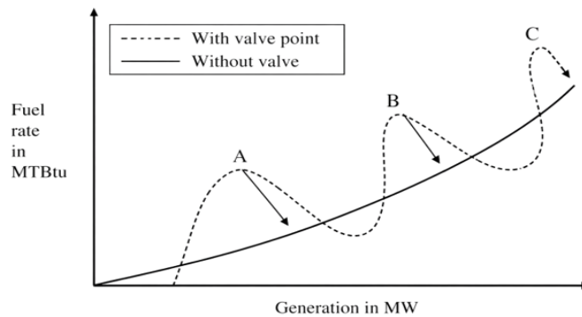
Figure 1. Valve point loading curve
