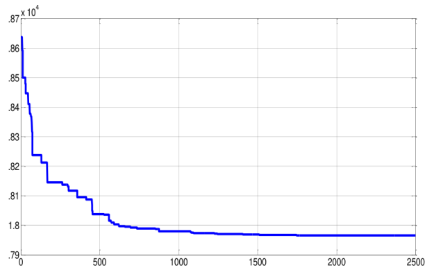
Figure 5. Convergence characteristics of BSA for 13 unit system with valve point loading effect.
