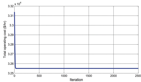
Figure 6. Convergence characteristics of BSA for 15 unit system with POZ and ramp rate limit.
