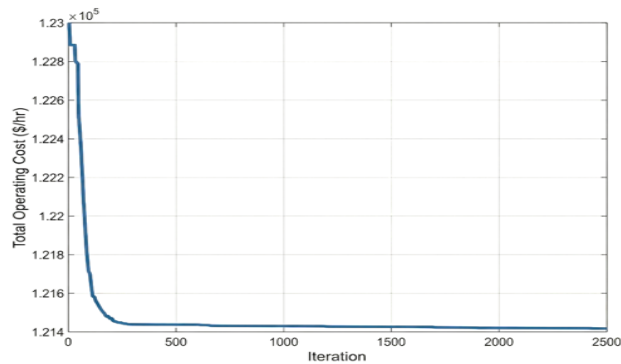
Figure 7. Convergence characteristics of 40 unit system with valve point loading effect.
