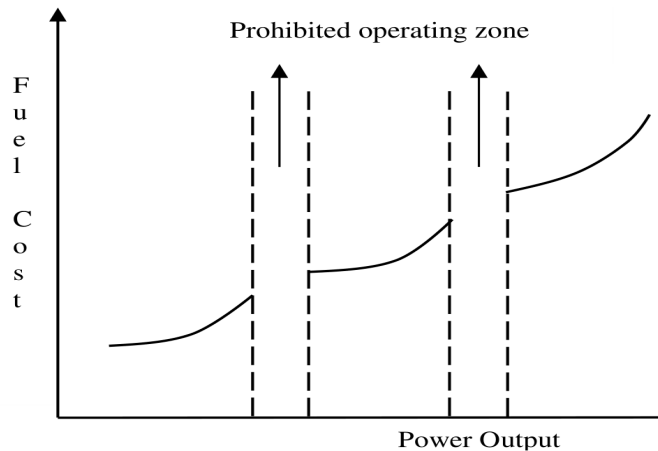
Figure 2. Input-output curve with prohibited operating zones.
