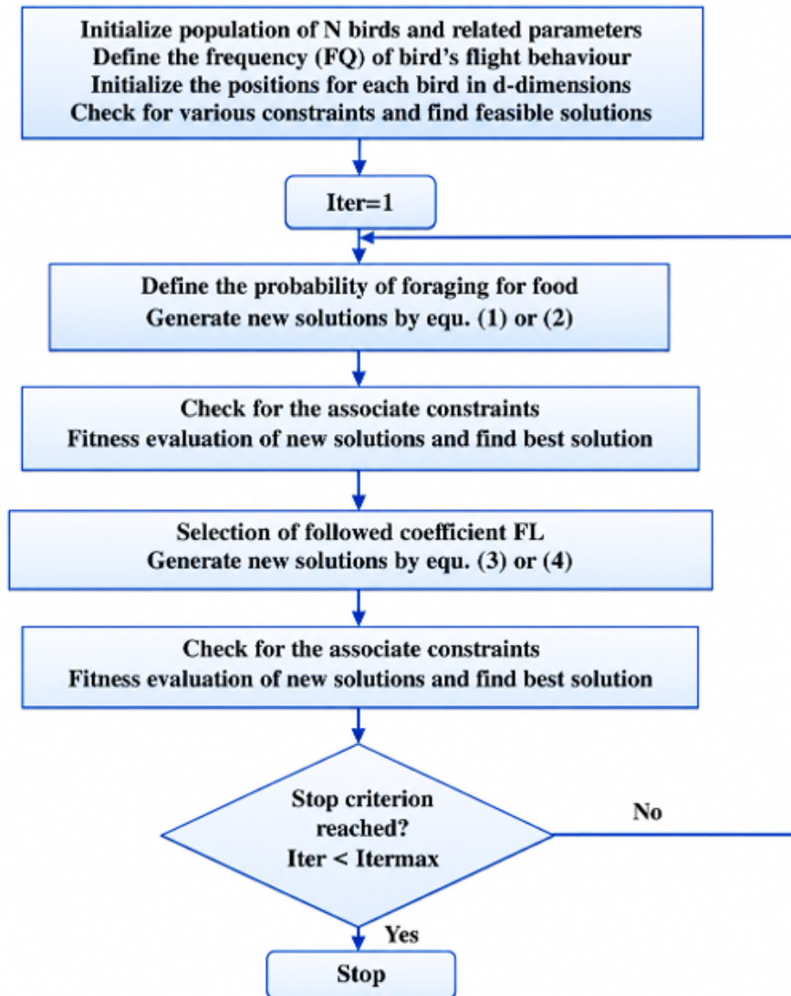
Figure 3. Flow chart of BSA for ELD problems
