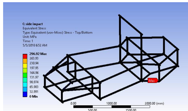
Figure 9. Stress applied at Rear due to impact
