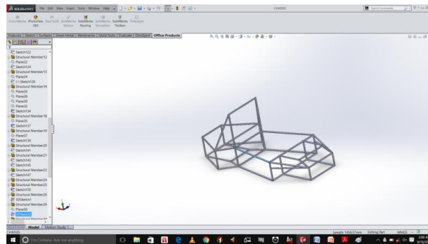
Figure 7. Isometric view for the frame
