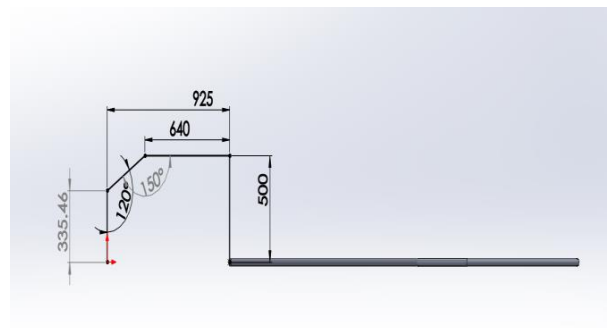
Figure 3. Side view with measurements
