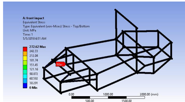
Figure 8. Stress applied at Front due to impact
