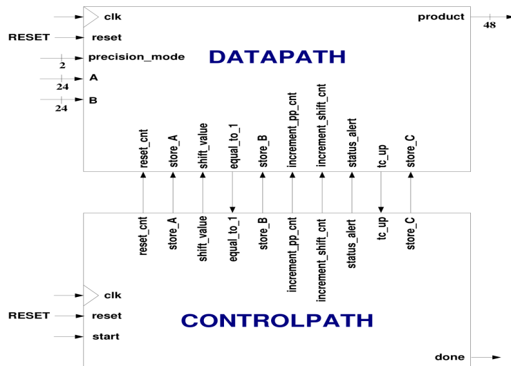
Figure 2. FSM-D Model for Novel 24-bit Binary Multiplier for Single Precision Floating Point Multiplication
