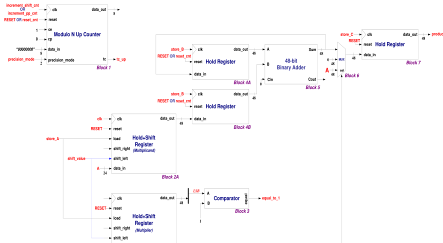
Figure 1. Datapath Design for Novel 24-bit Binary Multiplier for Single Precision Floating Point Multiplication
