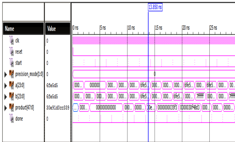
Figure 3. I Sim Simulation for Novel 24-Bit Binary Multiplier Architecture
