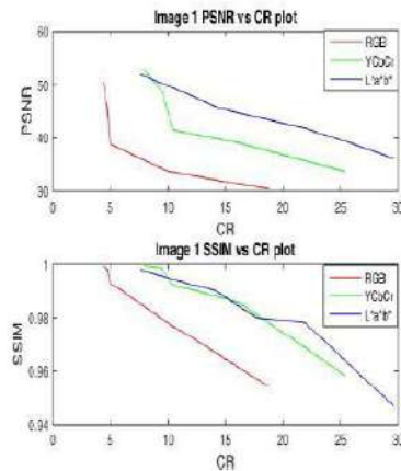
Figure 6. Variation of PSNR and SSIM vs. CR for different approaches of compression for test image 1.
