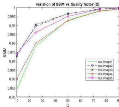
Figure 4. Variation of SSIM versus Quality factor ( Q ).
