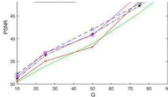
Figure 3. Variation of PSNR versus quality factor ( Q ).
