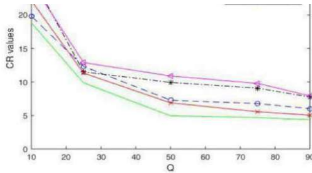
Figure 5. Variation of Compression Ratio (CR) versus Quality factor (Q).
